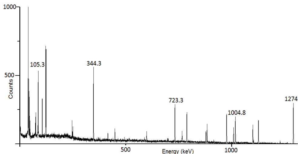
Figure 2 Europium spectrum
